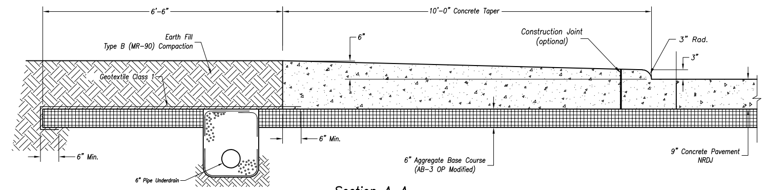
Section A-A (Concrete Roadway) Not to Scale
