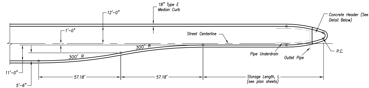
Typical Left Turn Lane Not to Scale
