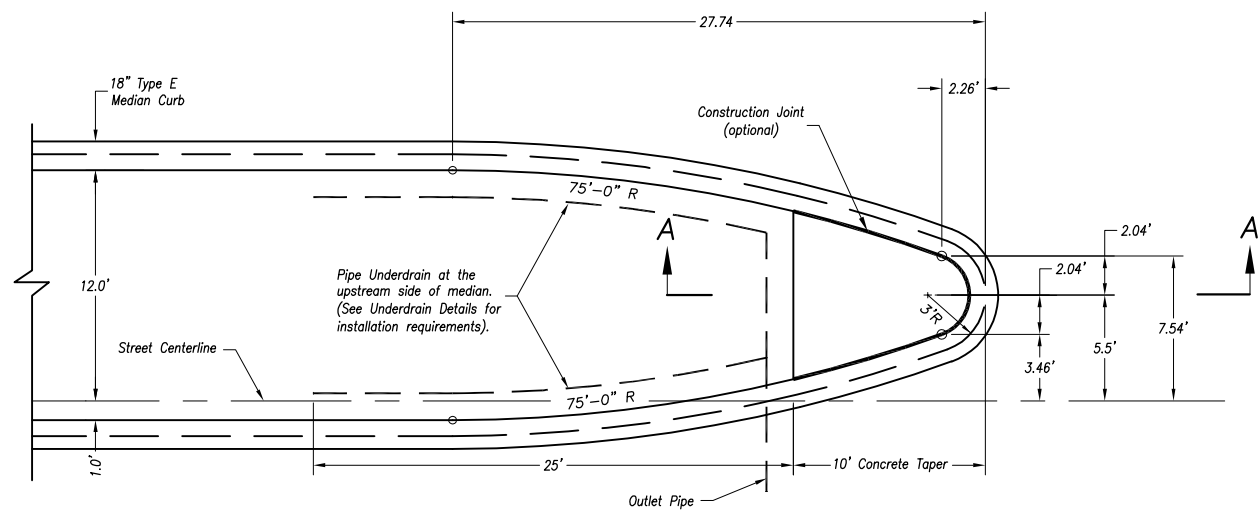
Typical Median Bullet Nose Detail Not to Scale
