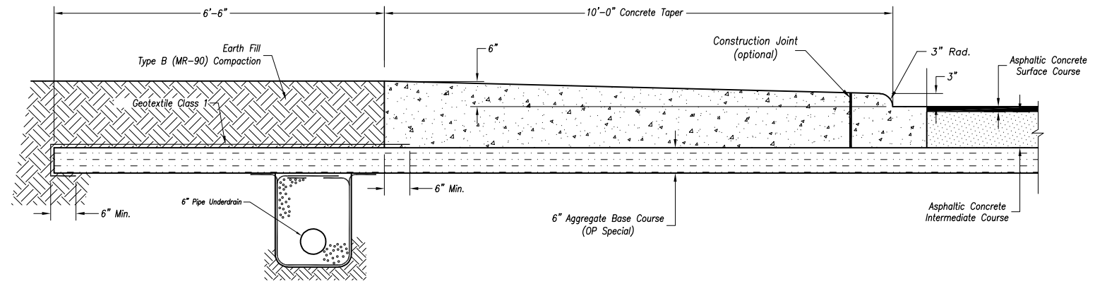
Section A-A (Asphalt Roadway) Not to Scale
