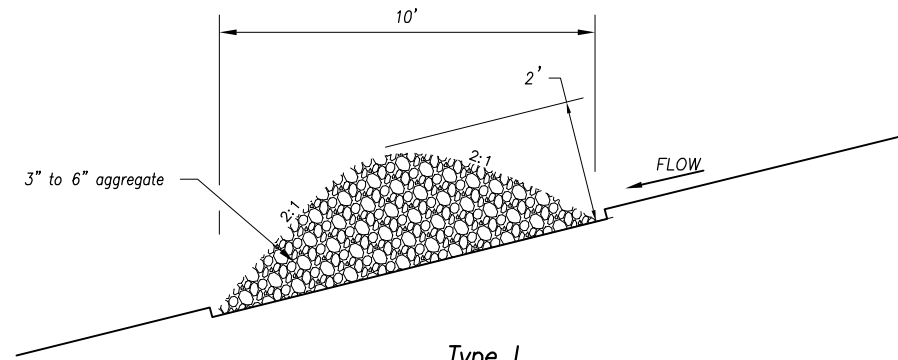
Type I (2 Acres or less of Drainage Area) Not to Scale
