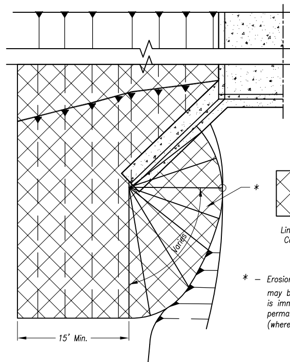
Partial Box Culvert Plan
