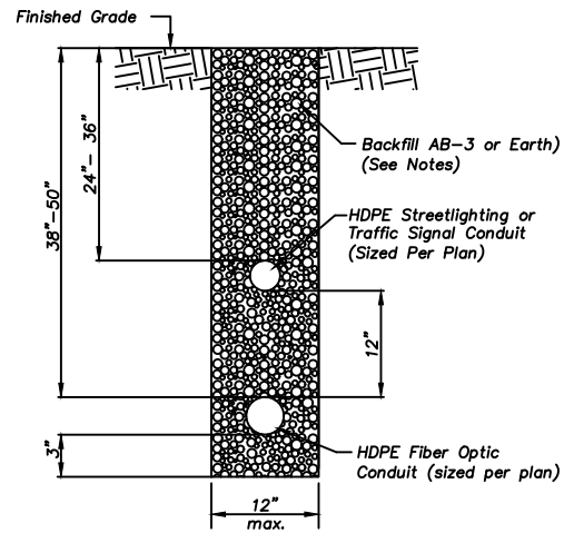
Trench in Unpaved Areas
