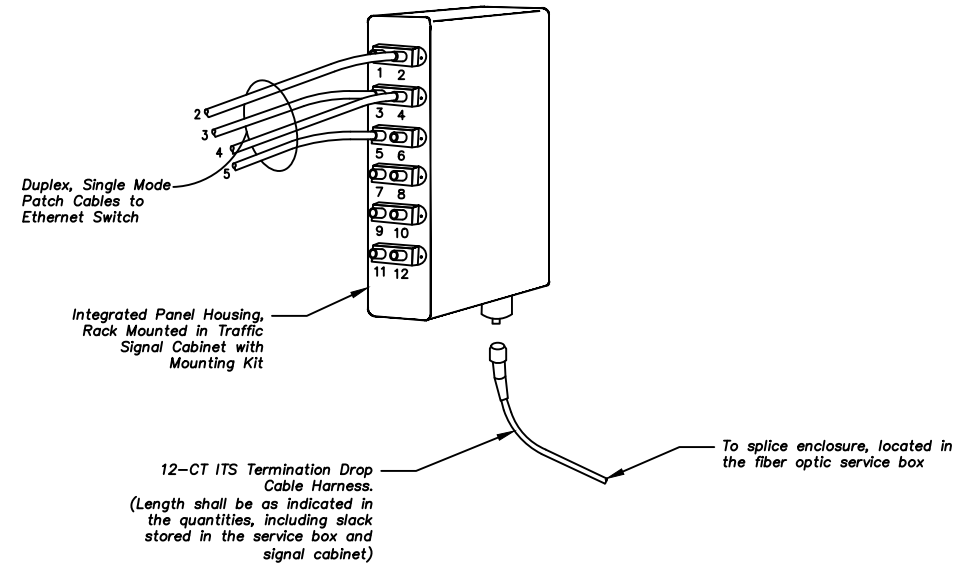
12-CT ITS Termination Drop Cable Assembly
