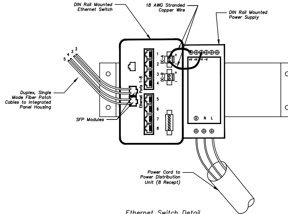
Ethernet Switch Detail
