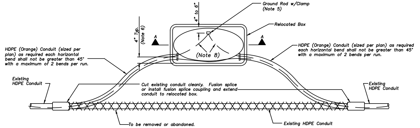
Plan (Conduit Position) Relocated Box Installation Detail
