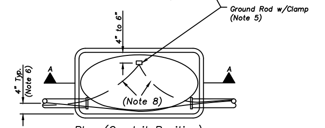
Plan (Conduit Position) Straight Through Run
