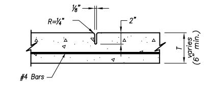
Contraction Joint
