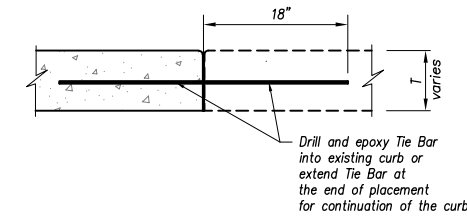
Construction Joint
