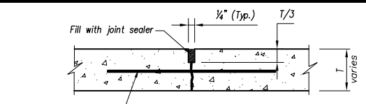
Logitudinal Tied Joint
