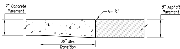
Isolation Joint at Residential Asphalt Street
