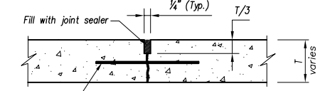
Logitudinal Tied Joint
