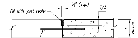
Logitudinal Construction Joint
