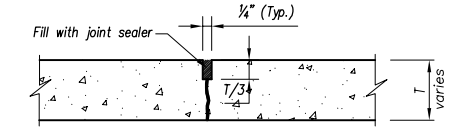
Untied Contraction Joint
