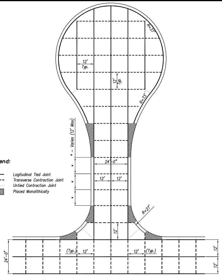
Typical Residential CDS (*)
