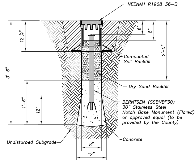
MONUMENT AND BOX WITH COMPACTED BACKFILL
