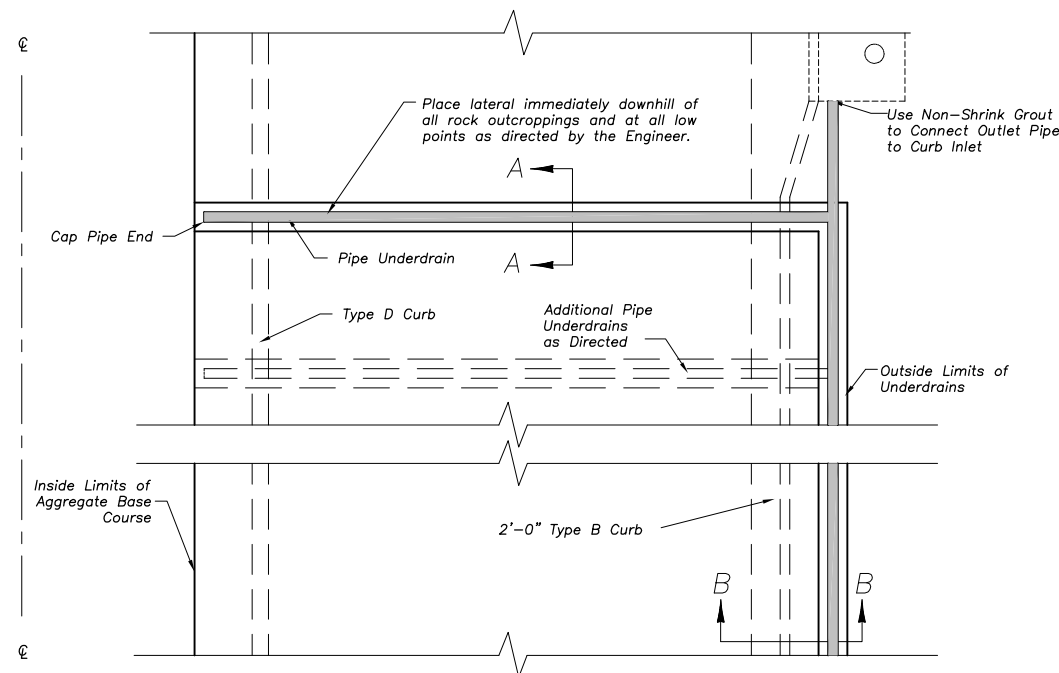
UNDERDRAIN LAYOUT
